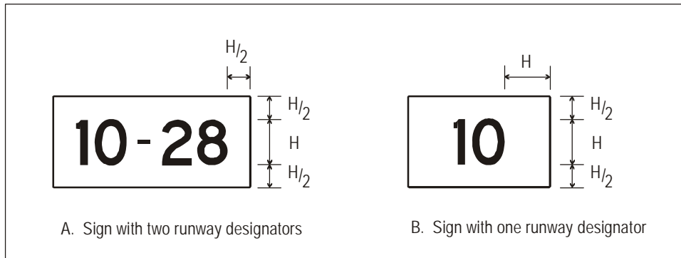
Figure A4-4. Sign dimensions
